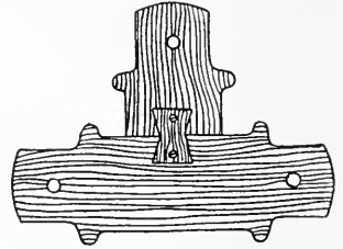
FIG. 569. COPED JOINT DETAILED.
